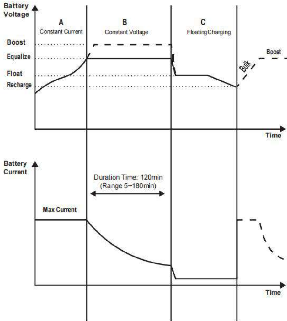
Battery Changing Stage Curve
